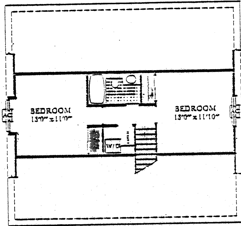
SECOND FLOOR
